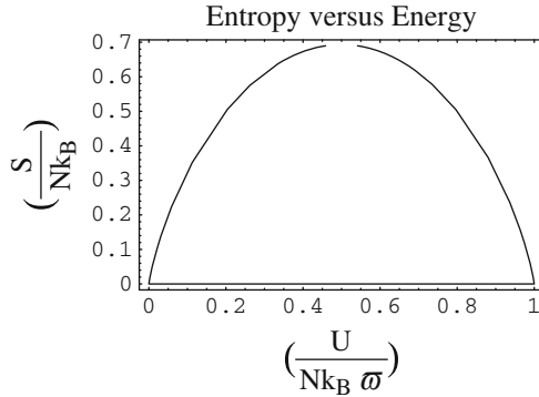
Fig. 11.16 Entropy S , in units of Nk_B , as a function of the Energy U , in units of Nk_B \varpi , for a two state nuclear paramagnet. The shown value of the entropy is equal to zero at both the minimum value of the energy – i.e., at U = 0 – and the maximum value – i.e., at U = Nk_B \varpi . The entropy rises with the increase in temperature and seems to level off at its maximum value of Nk_B \ln\{2(\frac{1}{2}) + 1\} = Nk_B \ln\{2\} . Recall that S(T) is symmetric with respect to the temperature: that is, S(+T) = S(-T) . At the position marked by a small empty space in the otherwise continuous looking curve, the derivative (\frac{\partial S}{\partial U})_{V,N} changes its value from (+0) to (-0) , which indicates that at this point the temperature instantly changes from (+\infty) to (-\infty) . Note that the derivative \left(\frac{\partial(\frac{S}{Nk_B})}{\partial(\frac{U}{Nk_B \varpi})}\right)_{N,V} is equal to (\frac{\varpi}{T}) – and its positivity from the position U = 0 to (\frac{U}{Nk_B \varpi}) = 0.5 indicates positive values of the temperature while its negativity in the range (\frac{U}{Nk_B \varpi}) = 0.5 \rightarrow 1 indicates negative values for the temperature. From left to right the temperature increases according to (T = 0 \rightarrow +\infty, -\infty \rightarrow -0)
