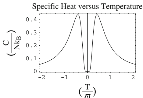
Fig. 11.17 The specific heat of the two-state nuclear paramagnet. At T = (+0) the specific heat, as also shown in Fig. 11.10, is equal to zero – which is its minimum value. It rises – first slowly and then rapidly – with the increase in temperature and, as expected, undergoes a Schottky anomaly before trailing off toward its minimum value of zero as the temperature heads toward (+\infty) . Note that C(T) is symmetric with respect to the interchange of temperature: that is C(+T) = C(-T)
