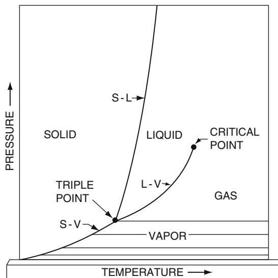
Fig. 10.1 Schematic plot of the Clausius–Clapeyron equations and the phase boundaries for real substances except \text{H}_2\text{O} [Copied with permission from Sears and Salinger, op. cit., figure 2-8 (a), p. 32]
