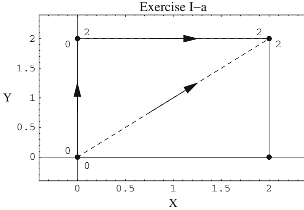
Fig. 1.1 Paths traveled. The paths traveled are: (First) : From the point (0,0) up to (0,2) and then to (2,2). (Second) : Another possibility is to travel directly from (0,0) across to the point (2,2)
