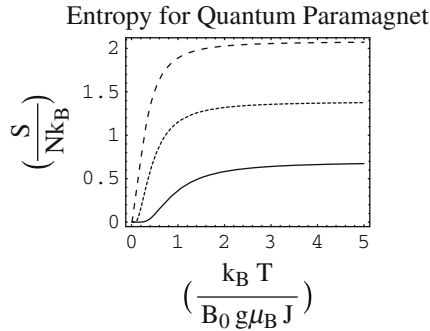
Fig. 11.7 Entropy of a Quasi-Classical Quantum Langevin Paramagnet as a Function of \frac{1}{x} = \left( \frac{k_B T}{B_0 g \mu_B J} \right) . The solid curve refers to J = \frac{1}{2} ; the short-dashed curve relates to J = \frac{3}{2} and the curve with slightly longer dashes is for J = \frac{7}{2} . Notice that at high end of the temperature scale, the curves are clearly heading toward their limiting value of \ln(2J+1) . The plots are in dimensionless units
