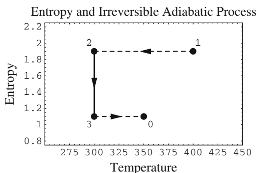
Fig. 4.4 Entropy/( J \cdot K^{-1} ) versus Temperature/ K . The scale shown is arbitrary. Broken lines are reversible adiabats and the full line is a reversible thermostat. The irreversible adiabatic process, that takes the system from the equilibrium state 0 to 1, passes through non-equilibrium states that cannot be displayed in the above plot. Note, S_3 = S_0 and S_2 = S_1 . Also, T_3 = T_2
