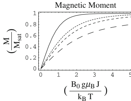
Fig. 11.8 The Ratio \left( \frac{M}{M_{\text{sat}}} \right) is Plotted as a Function of \left( \frac{B_o g\mu_B J}{k_B T} \right) . Here M represents the quasi-classical quantum statistical average of the system magnetic moment and M_{\text{sat}} its saturation value. The temperature is T and the magnetic field is B_o . The solid curve refers to J = \frac{1}{2} ; the thinnest, dashed curve is for J = \frac{3}{2} ; the next lower curve refers to J = \frac{5}{2} ; while the lowest curve – with long dashes – represents the classical limit, i.e., J \rightarrow \infty . Notice that the solid curve has nearly reached its maximum possible value of unity when \left( \frac{B_o g\mu_B J}{k_B T} \right) \approx 3 . For a J = \frac{1}{2} system, this means that the magnetic moment is close to reaching saturation when k_B T falls below (B_o \mu_B)/3 : or equivalently, when the ratio \left( \frac{B_o}{T} \right) rises above the value \left( \frac{3k_B}{\mu_B} \right) = \frac{3 \times 8.617343(15) \times 10^{-5}}{5.788381755(79) \times 10^{-5}} (\text{eV} \cdot \text{K}^{-1} / \text{eV} \cdot \text{T}^{-1}) \approx 4.4662 \text{ T K}^{-1}
