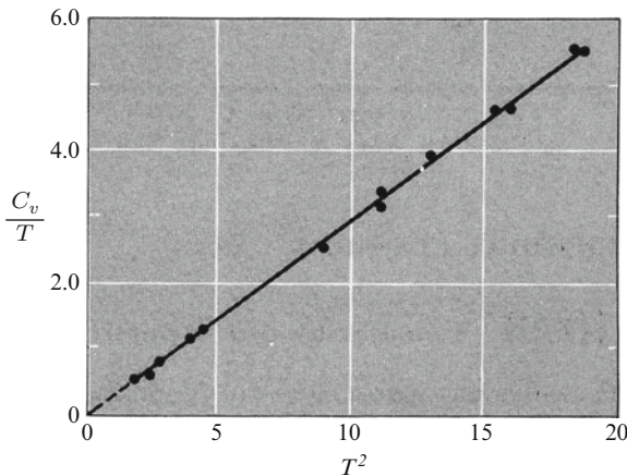
Fig. 11.19 As reported in Phys. Rev. 91, 1354 (1953), the plot presents the ratio \frac{C_v}{T} for KCl as a function of T^2 . Measurements are from Keesom, P. H., and Pearlman, N. Notice that there is no intercept. This indicates that at very low temperature, the specific heat varies as T^3 rather than as T . [The drawing is copied with permission from F. Reif's book: Fundamentals of Statistical and Thermal Physics, figure 10.2.3, p. 417, Waveland Press, Inc. (2009)]
