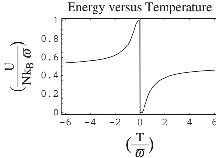
Fig. 11.14 Energy U , in units of Nk_B\varpi , as a function of temperature T , in units of \varpi , for a two state nuclear paramagnet. Notice that the energy is equal to zero – which is its minimum value – at T = (+0) . It rises with the increase in temperature and levels off at \left(\frac{Nk_B\varpi}{2}\right) as the temperature heads upward in the direction of T \rightarrow (+\infty) . Just beyond T = (+\infty) is T = (-\infty) . (Note, in theory, all negative temperatures are higher than +\infty .) From here, as the temperature moves “upwards” toward T = (-0) , the energy slowly rises above \left(\frac{Nk_B\varpi}{2}\right) and reaches its maximum value of (Nk_B\varpi) at the end of its journey at T = (-0)
