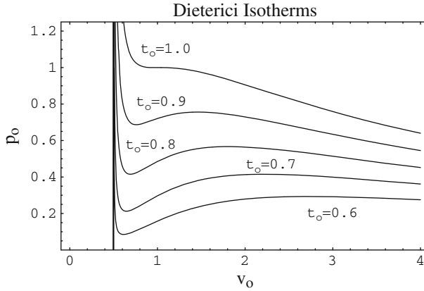
Fig. 6.9 Dieterici equation of state isotherms for t_o = 1.0, 0.9, 0.8, 0.7, 0.6
