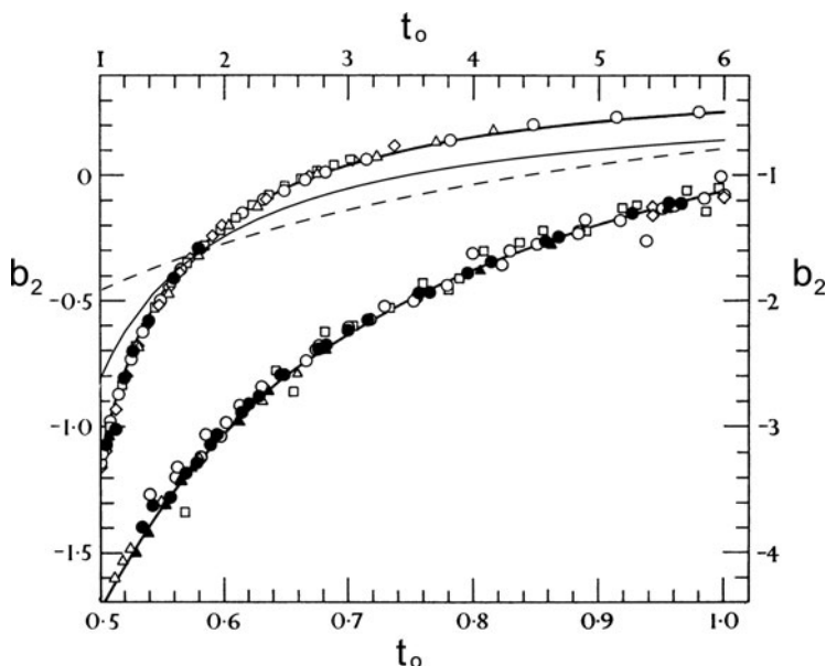
Fig. 6.6 Reduced second Virial coefficient \circ \bullet , Ar; \triangle \blacktriangle , Kr; \diamond , Xe; \square , \text{CH}_4 . For ease of display we have broken the data up into two parts. Experimental data shown on the lower curve refers to 0.5 \leq \frac{t}{t_c} \leq 1.0 . The right-hand and lower scales relate to the lower curve. The dashed curve represents the corresponding results of the Van der Waals theory. Data for 1.0 \leq \frac{t}{t_c} \leq 6.0 is displayed in the upper curve. The left-hand and upper scales relate to the upper curve. Full curve records corresponding Van der Waals results [Copied with permission from E. A. Guggenheim's book: "THERMODYNAMICS: An advanced treatment for Chemists and Physicists", figure 3.10, p. 137, North Holland Publishing Company, Amsterdam (1967).]
